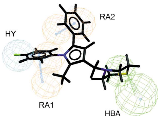
Figure 1. Compound 2 mapped to the pharmacophore model.
